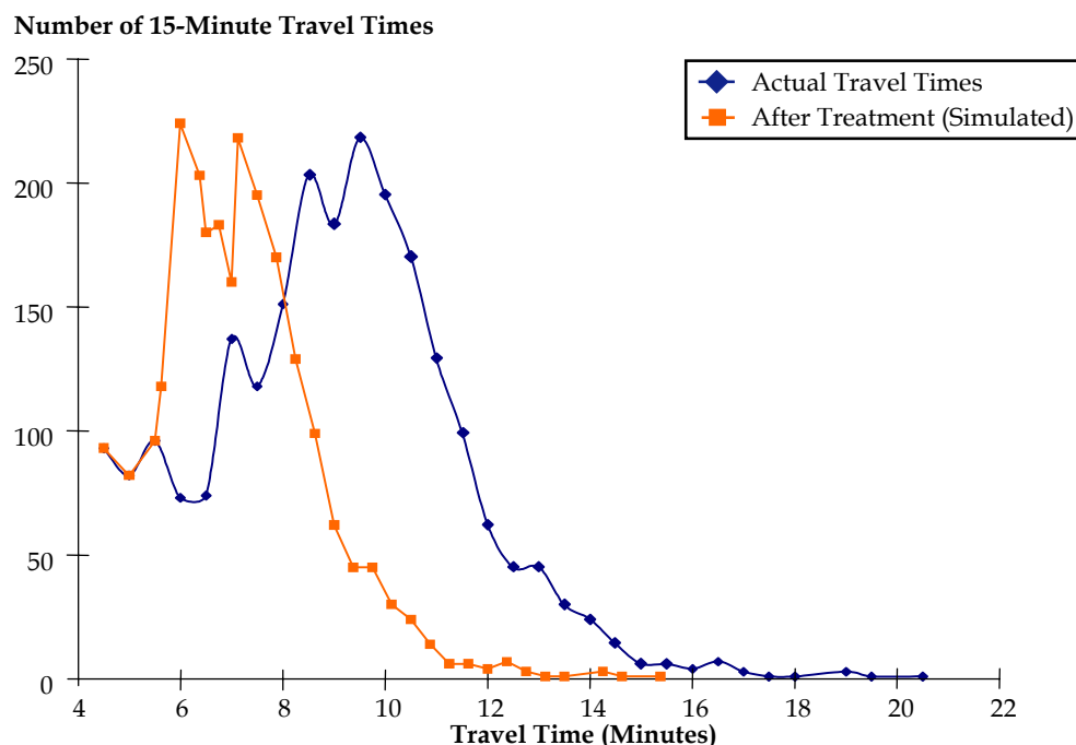
Figure 2.2 Actual and Improved Peak-Period Travel Times on I-75 Southbound Central Atlanta, 2002
